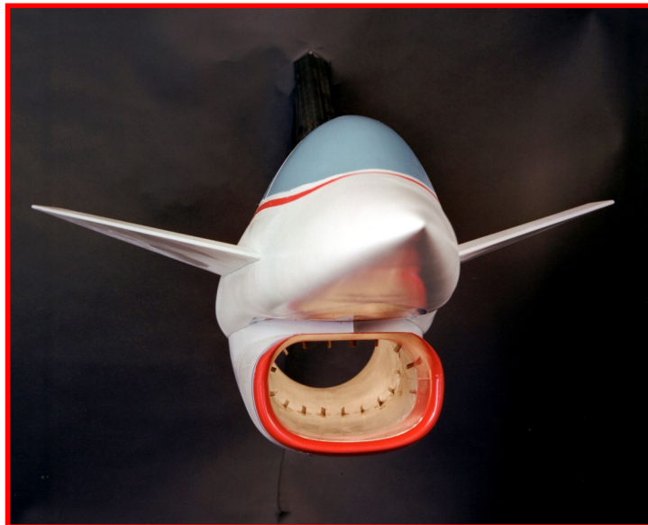
NASA's Lewis Research Center performed wind tunnel testing on a HiMAT inlet test model, as well as the J85-21 engine. Note the canard shape of this model.
