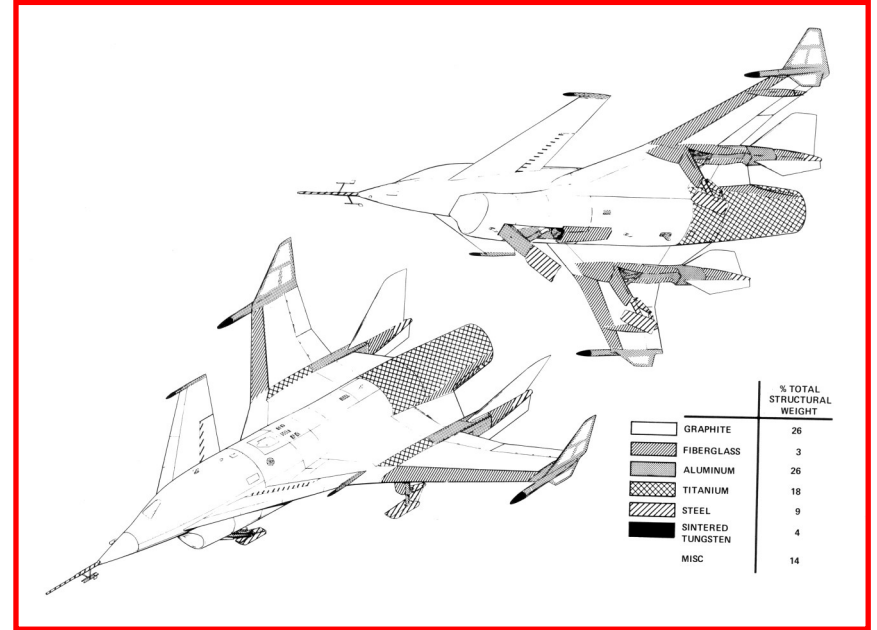
Graphic illustration showing the primary materials that went into the HiMAT vehicles. Graphite, aluminum and titanium make up the largest portions.
