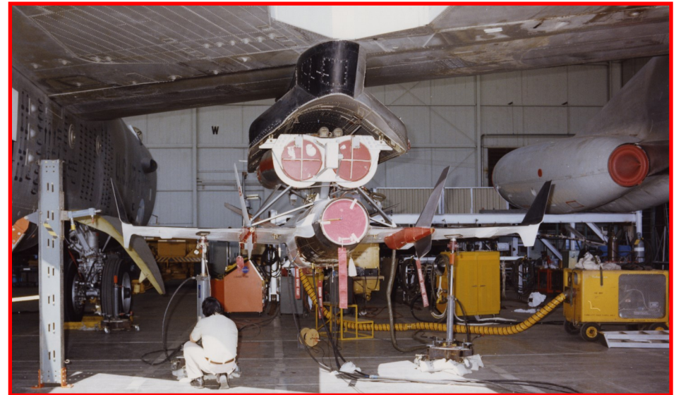
This series of photographs show HiMAT, RPRV 871, during NB-52B mating and calibration operations on April 22, 1982. In addition to new markings, ship 2 received new instrumentation on the upper wing and canard surfaces. All of this instrumentation required delicate calibration prior to its next flight.
