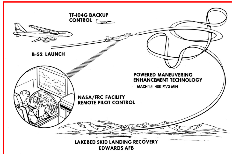
The illustration above shows the standard mission profile for a HiMAT test flight flown from a remote cockpit station. The small test vehicle measured just 23.5 feet (ft) in length and 15.6 ft wingspan as shown in the top illustration.
