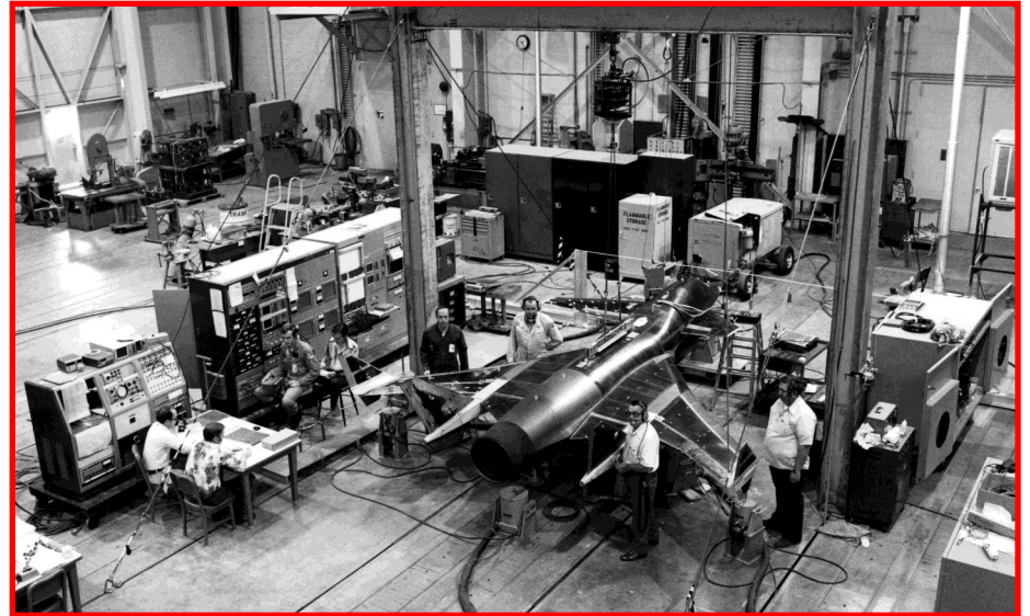
Ground Vibration Tests (GVT) are part of all new aircraft designs and both HiMAT aircraft endured this setup. Above, RPRV 871 during its GVT on November 15, 1978.
