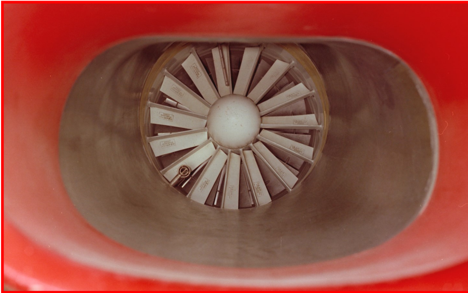
Looking down the inlet of HiMAT the GE J85 turbojet engine face is easily inspected by ground crew members.
