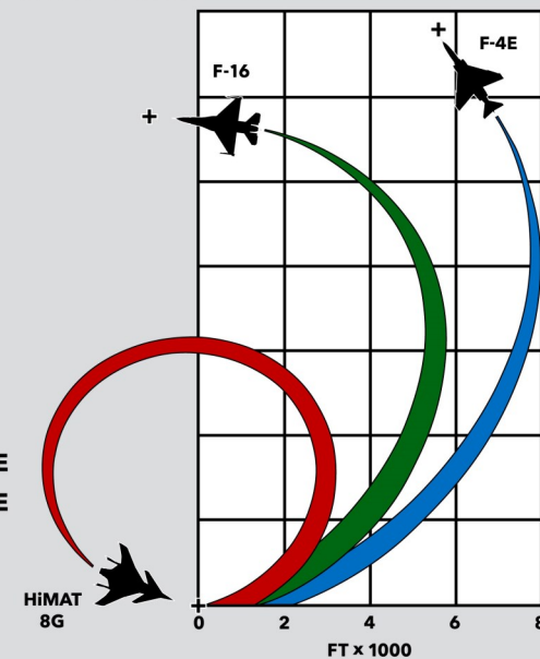
The illustration above compares the maneuverability and turning radius of HiMAT compared to fighter aircraft in service during the late 1970's.
