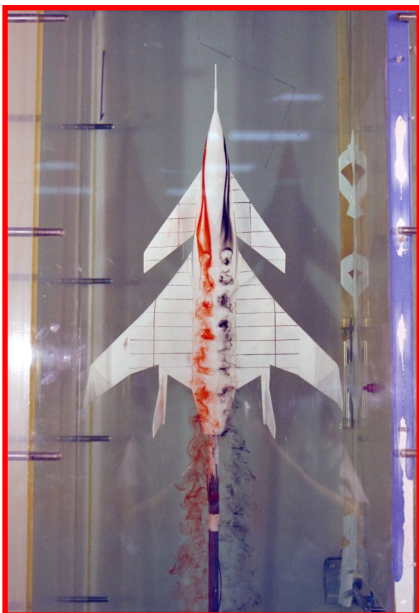
NASA tested a 1/15th scale HiMAT model in the water tunnel at Ames/Dryden Flight Research Facility during May 1979. Inexpensive water tunnel models made use of colored dyes injected into the water flow to visualize airflow under different flight conditions.
