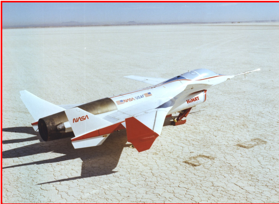
Completely repaired, RPRV 870 sits on Rogers Dry Lake after flight H1-6-13 on October 28, 1980. Two planned captive flight occurred on September 30 and October 10. All objectives were met during the second captive flight, though the main gear did not deploy when commanded during the first.
