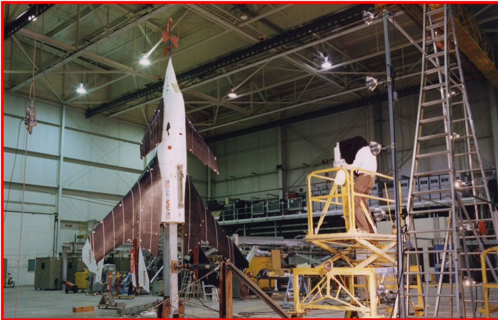
With the flight program over, the first HiMAT was placed in storage while the second was used for a series of composite aeroelasticity tests. These photos taken February 7, 1983, show RPRV 871 in the NASA ADFRF Loads Laboratory during photogrammetric measurement testing.
