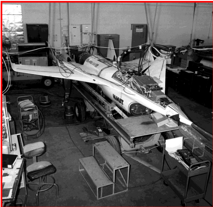
The condensed size of the avionics package used in HiMAT was due to the diminutive size of the HiMAT test aircraft. The compact nature added a degree of difficulty for the technicians that worked on the vehicle.
