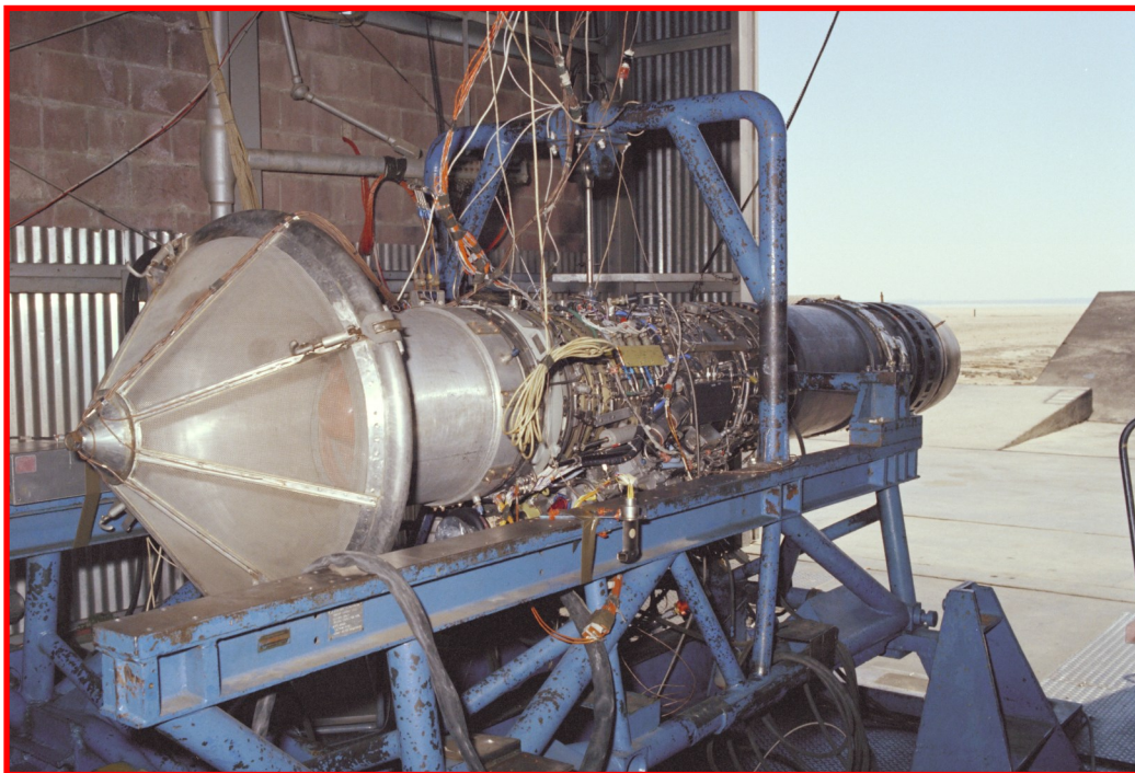
The GE J85 turbojet engine (above and left) used in HiMAT also powered the Northrop T-38 & F-5 family of aircraft, as well as the Cessna A-37 Drag-onfly. A compact design, the engine measured 112 inches in length and 20.8 inches in diameter at the inlet.
