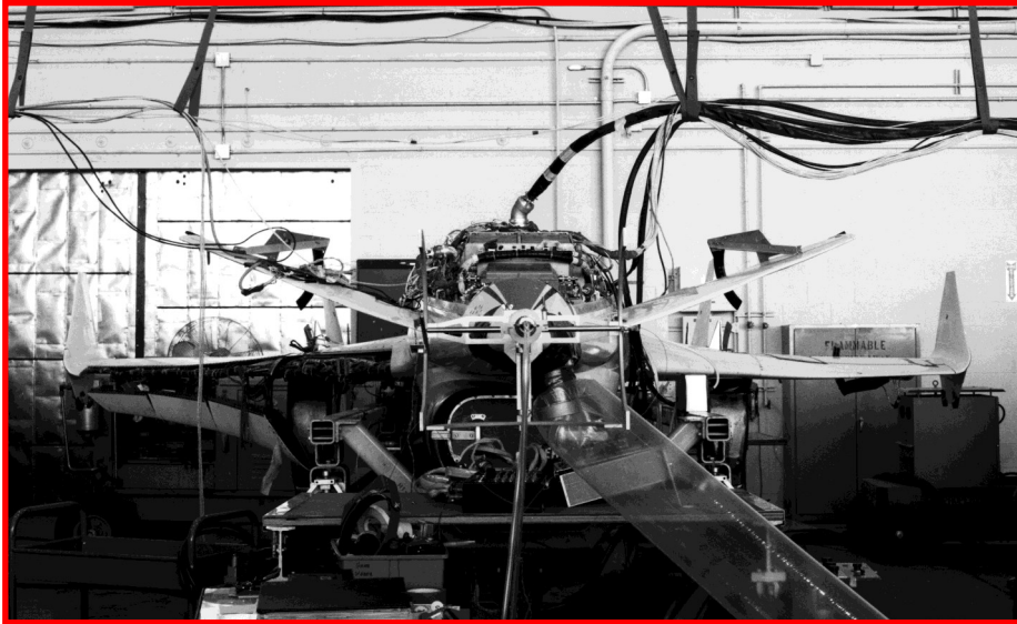
Looking like a patient on life support, RPRV 870 undergoes a series of systems tests in December 1978.
