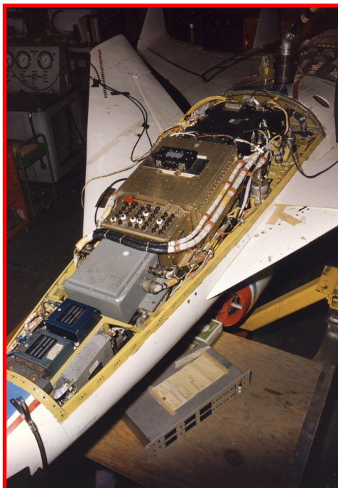
The condensed size of the avionics package used in HiMAT was due to the diminutive size of the HiMAT test aircraft. The compact nature added a degree of difficulty for the technicians that worked on the vehicle.
