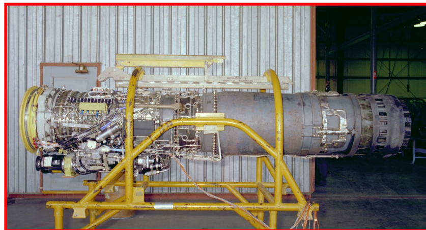
The GE J85 turbojet engine (above and left) used in HiMAT also powered the Northrop T-38 & F-5 family of aircraft, as well as the Cessna A-37 Drag-onfly. A compact design, the engine measured 112 inches in length and 20.8 inches in diameter at the inlet.
