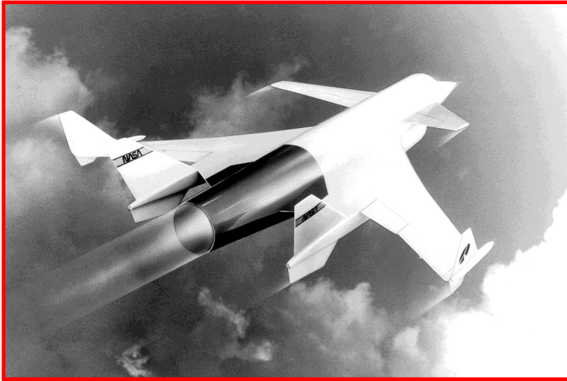
A refined artist concept from Rockwell, shows small pods on the outer wingtips that were not on the actual aircraft. Rockwell chose the General Electric (GE) J85 jet engine to power HiMAT.
