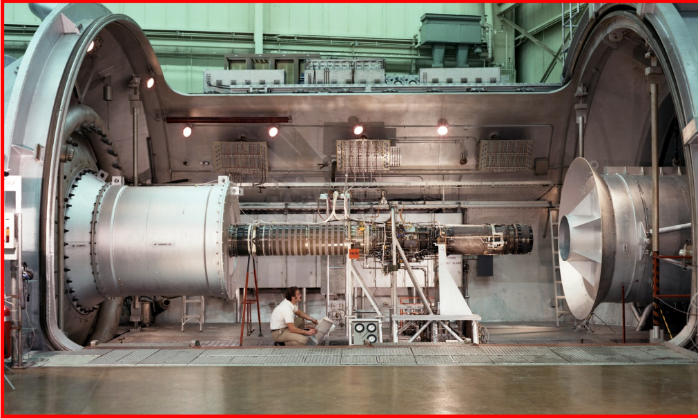
The GE J85-21 turbojet engine for HiMAT underwent extensive testing at the NASA Lewis Research Center in Cleveland, OH. The small engine weighed in at 684 pounds, yet produced 3,500 pounds thrust at military power and 5,000 pounds thrust in afterburner.
