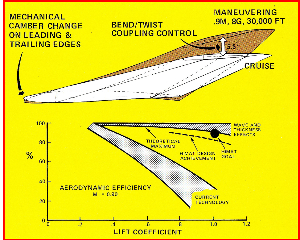
Predicted HiMAT composite wing bend and twist measurements during an 8G windup turn at 30,000 feet
