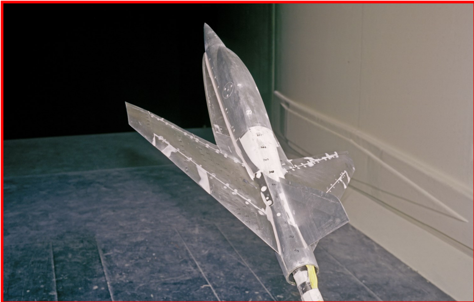
After proving the design of composite, aeroelastic wings on HiMAT, NASA applied the concept to more futuristic designs, such as this forward swept wing model.
