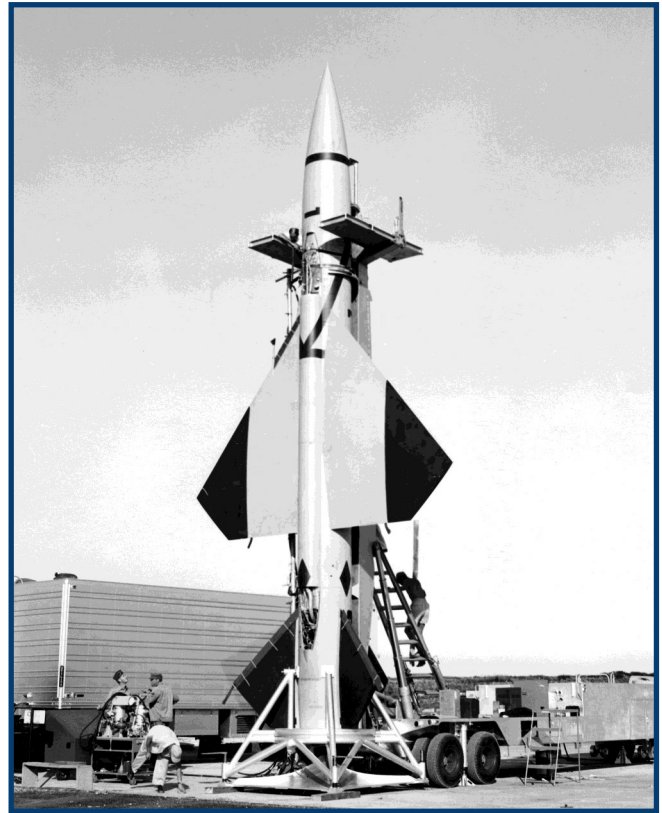
Top: First flown in 1952, the Boeing BOMARC ( B Oeing M ichigan A erospace R esearch C enter) originally carried an F-99 designation, but this changed three years later to IM-99. The XF-99 shown above had the vertical stabilizer on the bottom and did not yet incorporate the ramjet engines for cruise flight.
