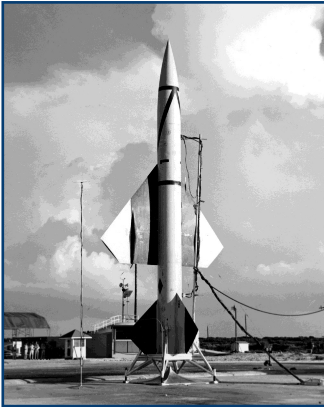
Top: First flown in 1952, the Boeing BOMARC ( B Oeing M ichigan A erospace R esearch C enter) originally carried an F-99 designation, but this changed three years later to IM-99. The XF-99 shown above had the vertical stabilizer on the bottom and did not yet incorporate the ramjet engines for cruise flight.
