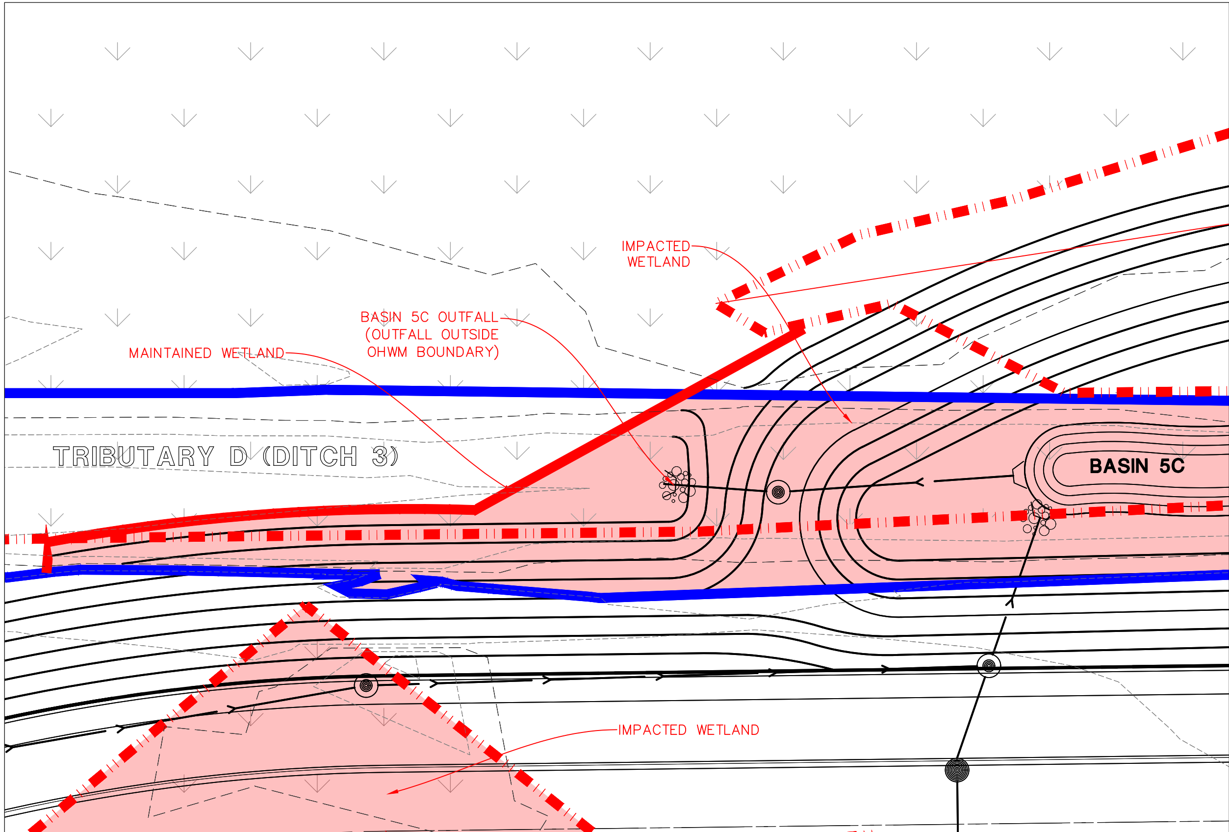
OUTFALL DETAIL G
