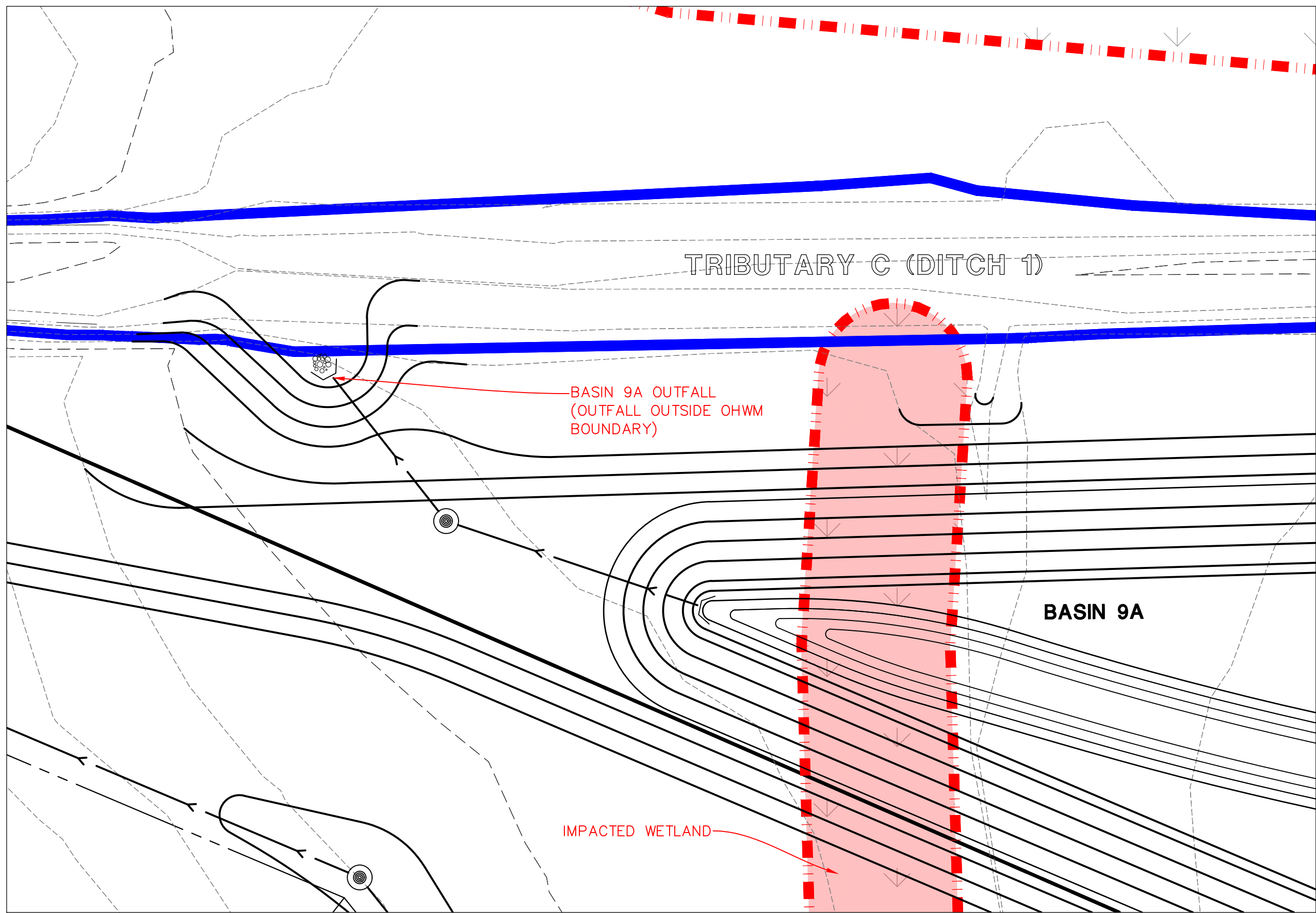
OUTFALL DETAIL C
