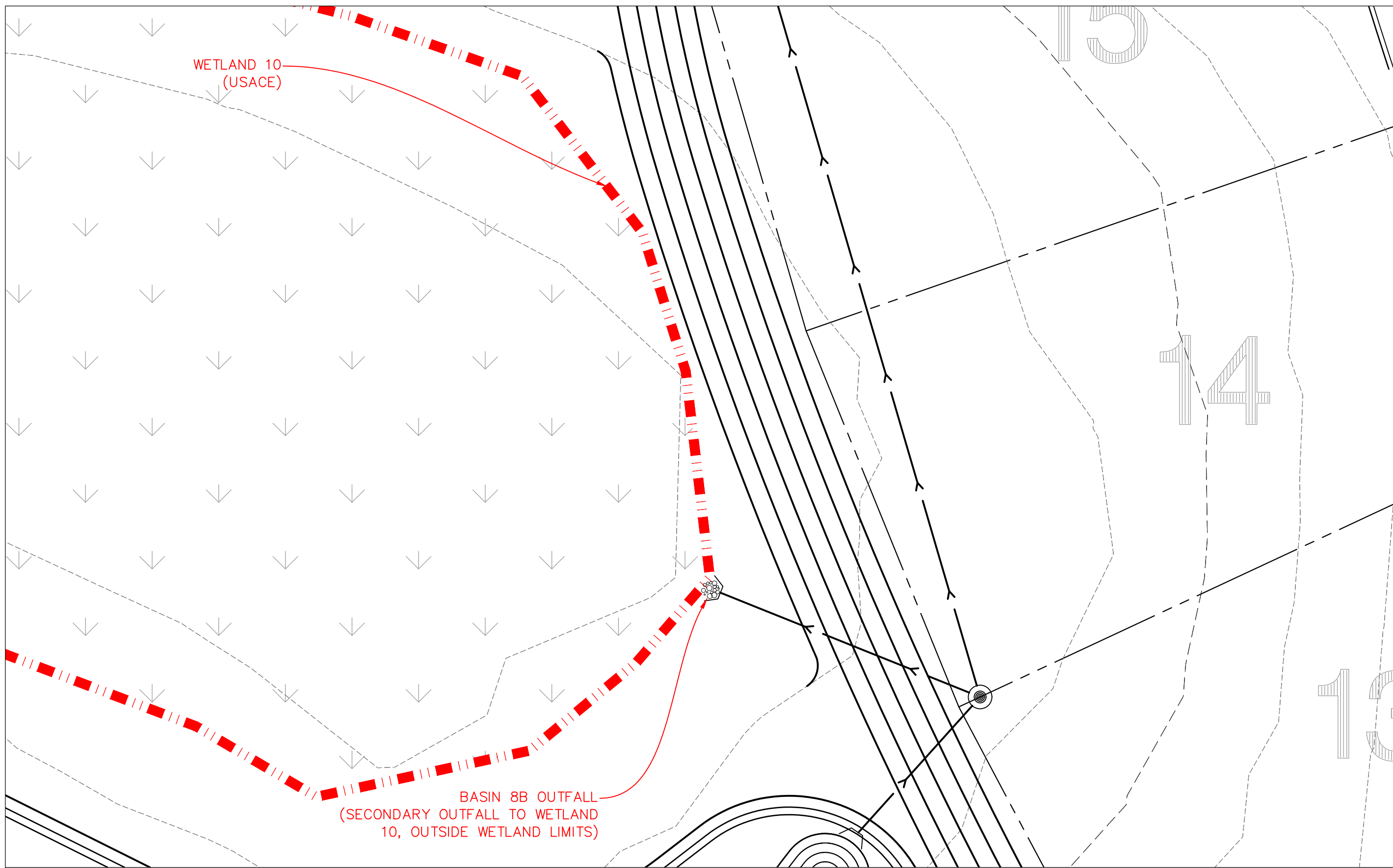
OUTFALL DETAIL D
