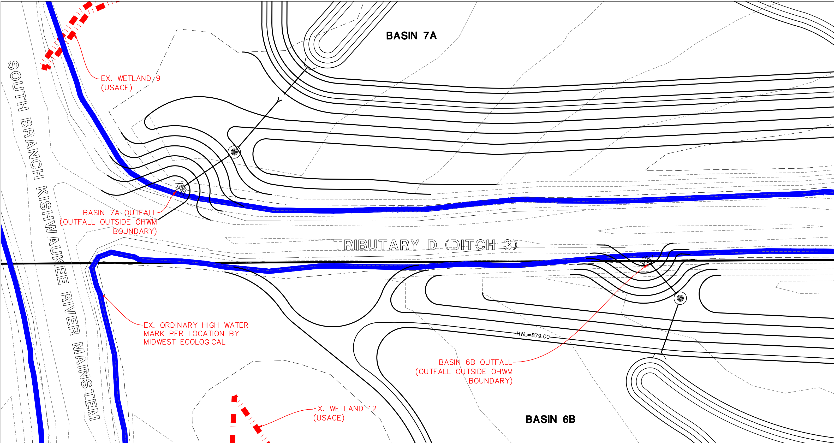
OUTFALL DETAIL E
