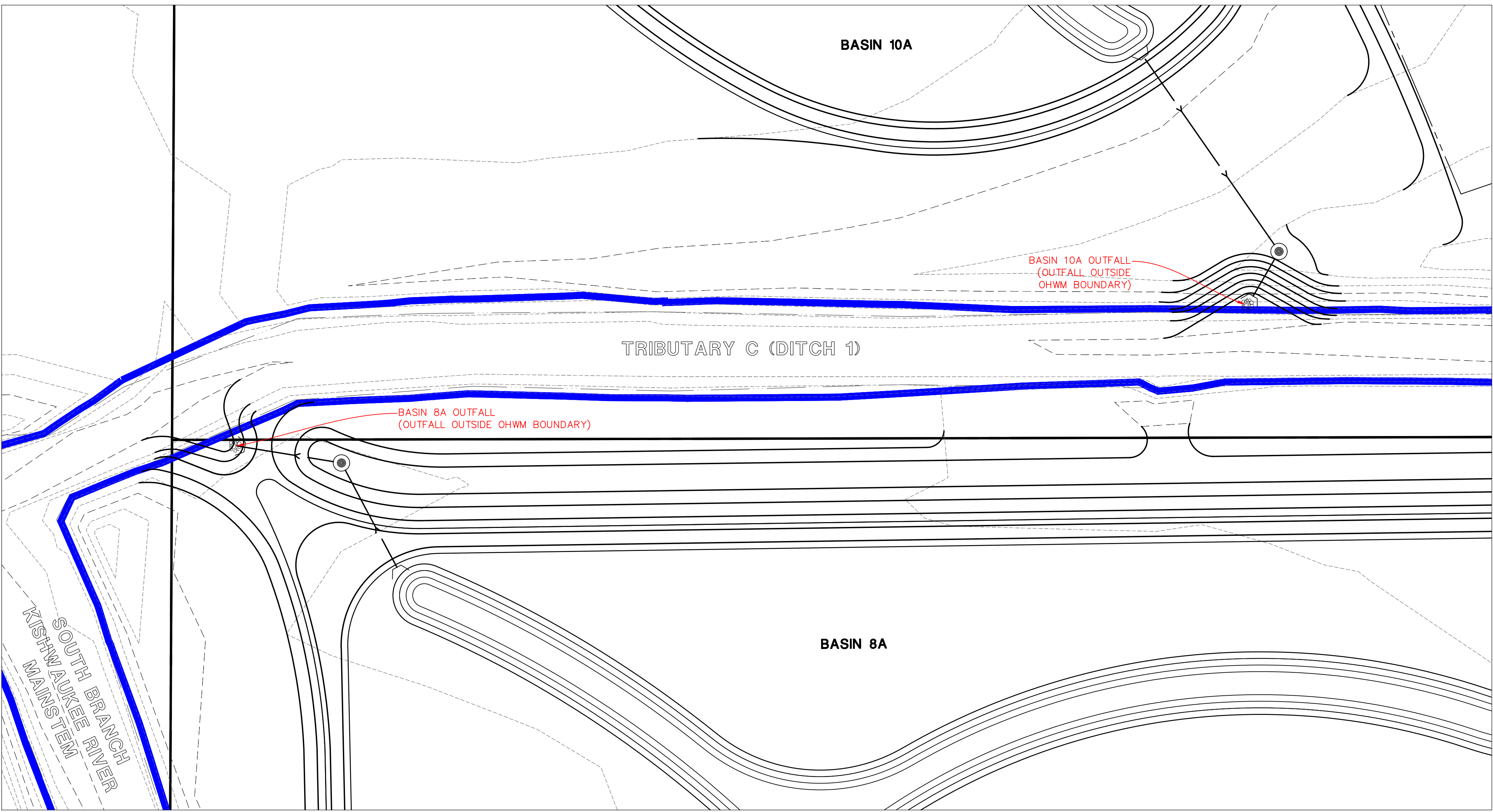
OUTFALL DETAIL A
