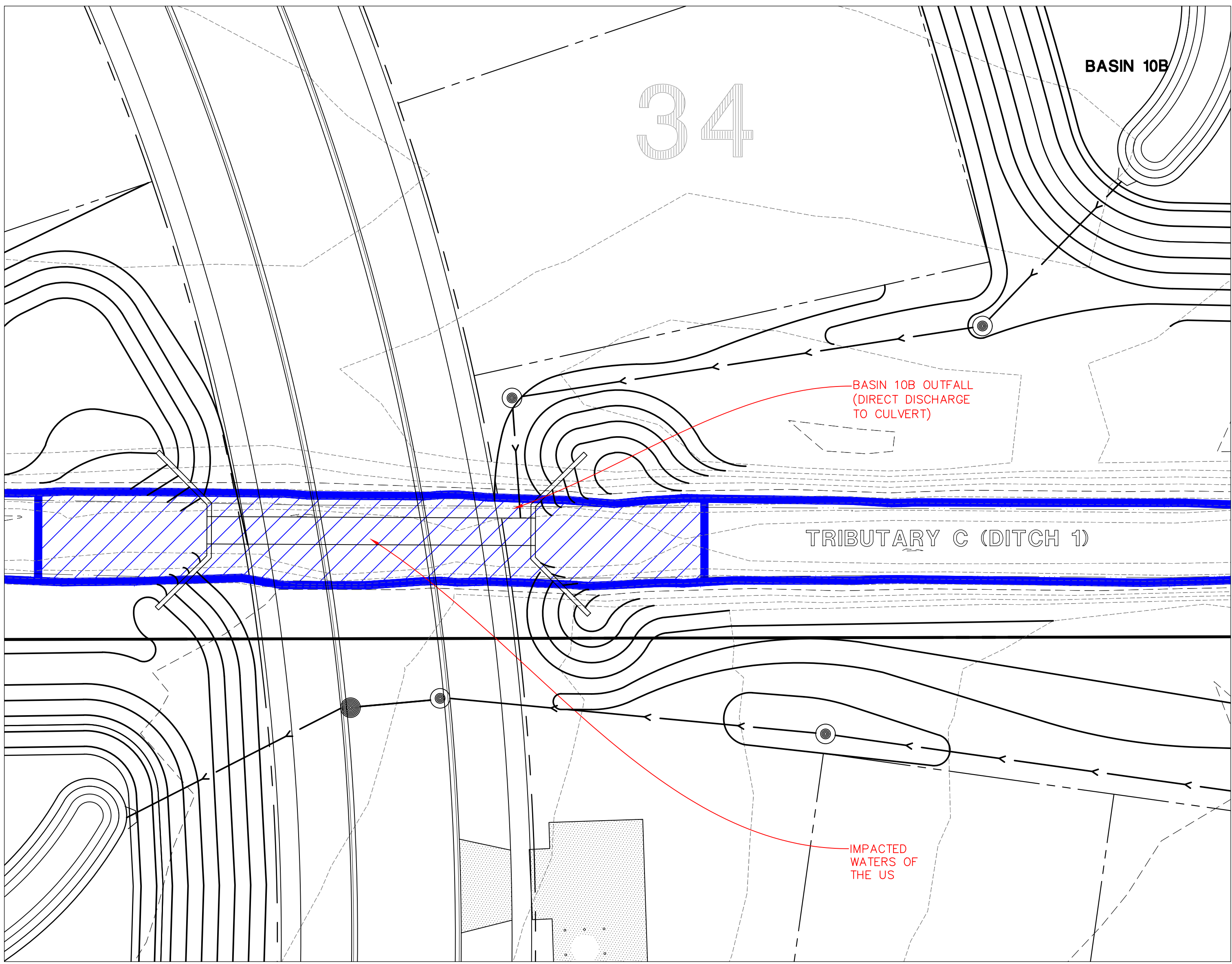
OUTFALL DETAIL B
