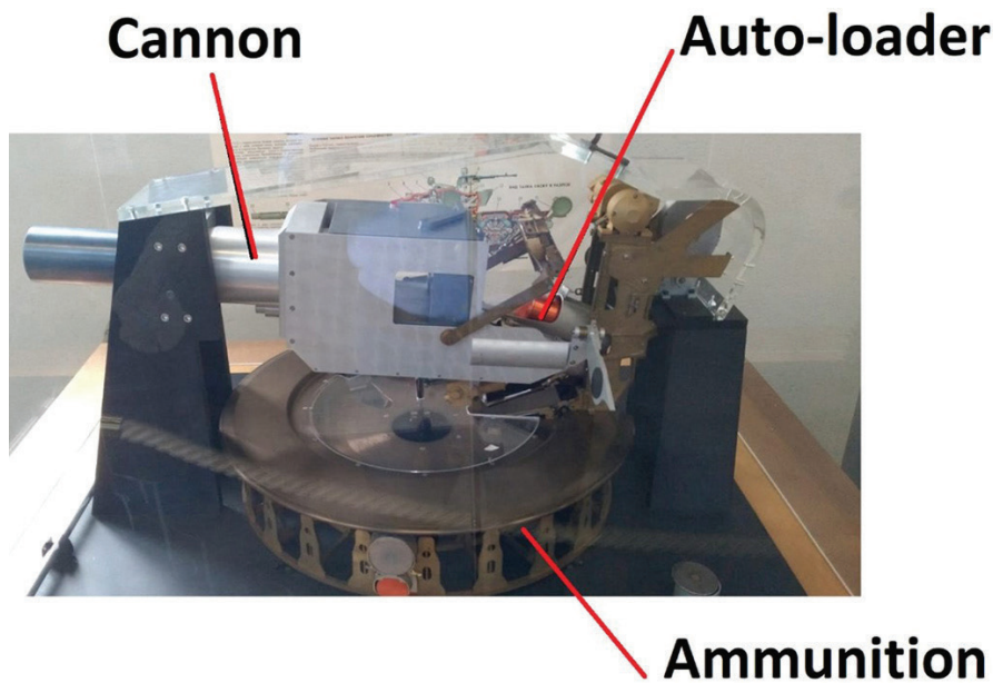
Figure 3. Mock-up of the Russian T-72 auto-loader displayed in France's Armor Museum. The ready-to-use-shells (there are 22) were severely criticized for causing the destruction and ejection of the turret when the tank is hit. However, with little storage space available in the tank, the crew is forced to place the other 17 projectiles elsewhere, like in the turret's interior wall, which make them much more dangerous than those placed in the floor. (Photo by MAJ Gonzalo Baez)
