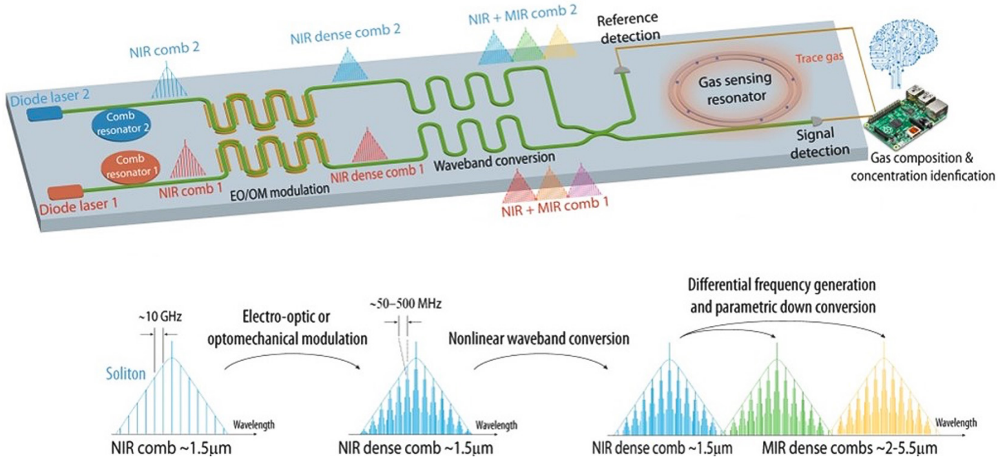
Schematic of the interleaved difference frequency generation (iDFG) dual-comb spectroscopy (DCS) setup. (Caltech image by Kerry Vahala)
