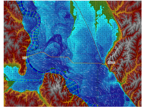
An inundation map created by the USACE Hydrologic Engineering Center River Analysis System (HEC-RAS) hydraulic modeling software. The solid green lines show waterway cross section while the short white marks indicate water flow during a flood event.
