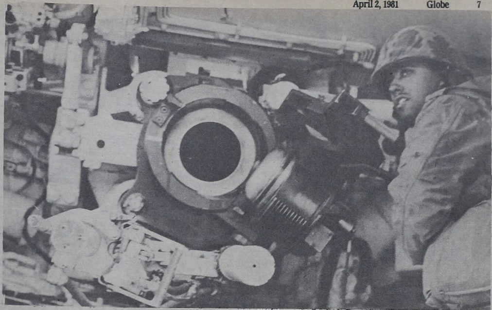
OPEN WIDE — Inside one of Battery O's self-propelled 105mm howitzers, LCpl. C.E. Robertson opens the breech preparing to load a round for a fire mission.
