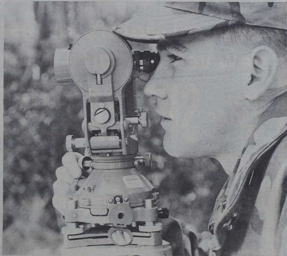
Corporal Kevin Shaffer, instrumentman, sights through a theodolite to a target at his next station.
