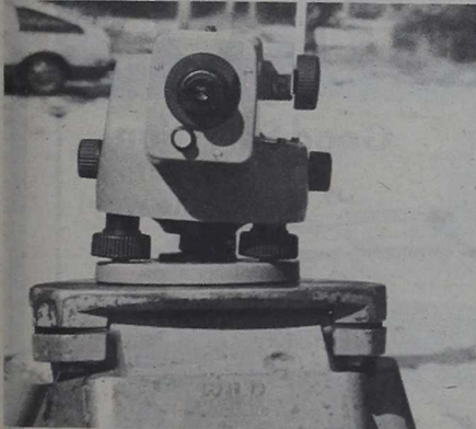
The automatic level is used for sighting on a graduated level rod to record differences in land elevations.
