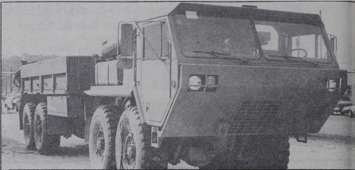
A Logistics Vehicle System sits outside the training lab at MCSSS motor transport school. The students will use this vehicle for hands-on application for their schooling, as necessary. (Photo by Cpl. Timothy P. Dougherty)
