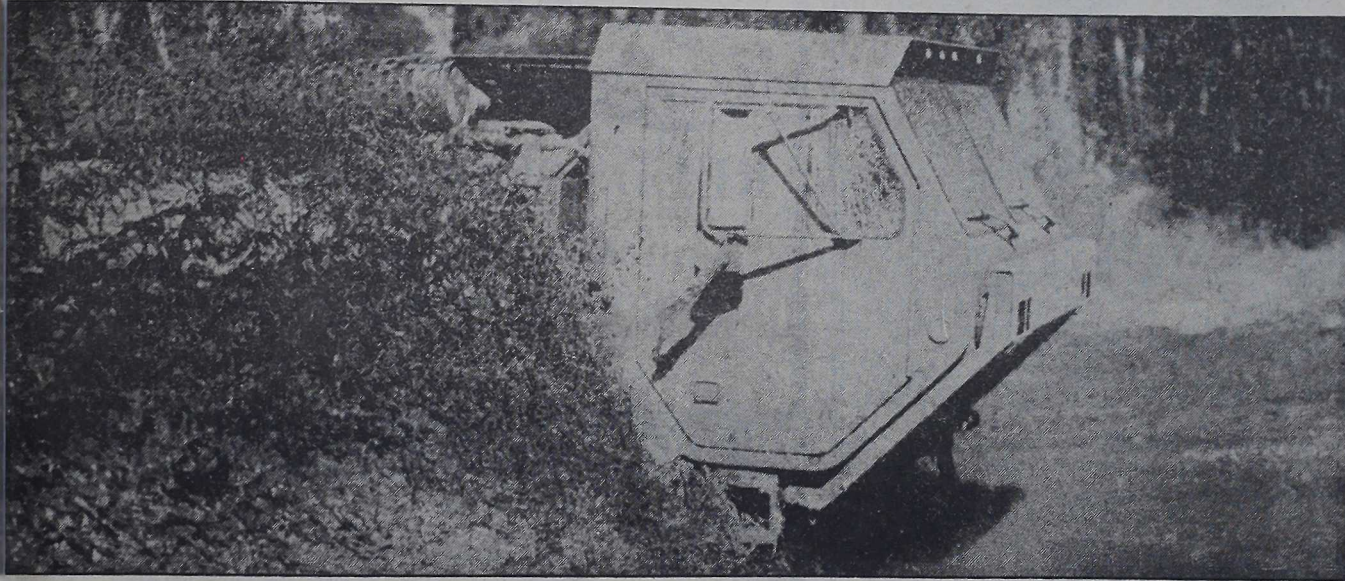
A fully-loaded Logistics Vehicle System makes its way through one of many mud-holes and water obstacles during the 6th MAB field exercise Combined Arms Operation-87. Proving that the vehicle could go anywhere and do anything, the Brigade Service Support Group-6 fleet of LVSs came through its first field test with flying colors. (Photo by Sgt. Rodney Germain)
