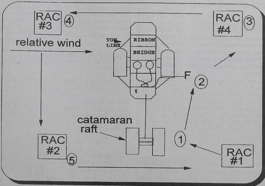
The boats to be resupplied form a perimeter around the Ribbon Bridge Raft. Starting with Boat #1, they rotate counter-clockwise filling up on ammunition from the towed catamaran raft, then pull up and get resupplied with fuel and other necessities from the Ribbon Bridge Raft. Each boat rotates into the position of the boat in front of it. If the wind is blowing the opposite direction, the rotation would go clockwise.
