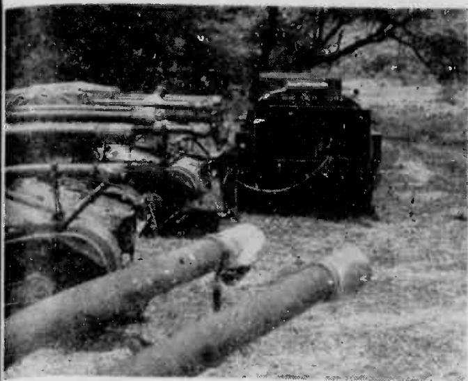
REFUELING —Crewmen and a supplyman pump 47 gallons of gas into an Ontos. An economical six cylinder engine permits a 150-mile cruising radius, an important factor offsetting fuel scarcity under combat conditions. Its top speed is over 30mph.
